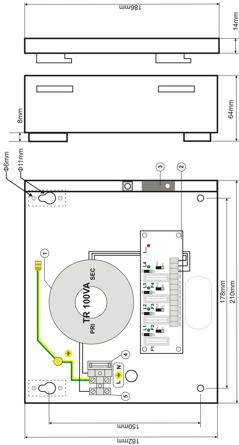
Fig.4. The view of the PSU.
