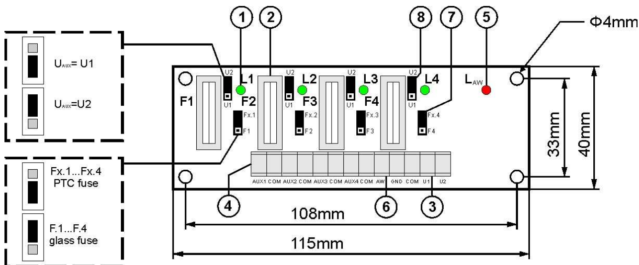
Fig.2. View of the LB8/24/27/AW strip.
