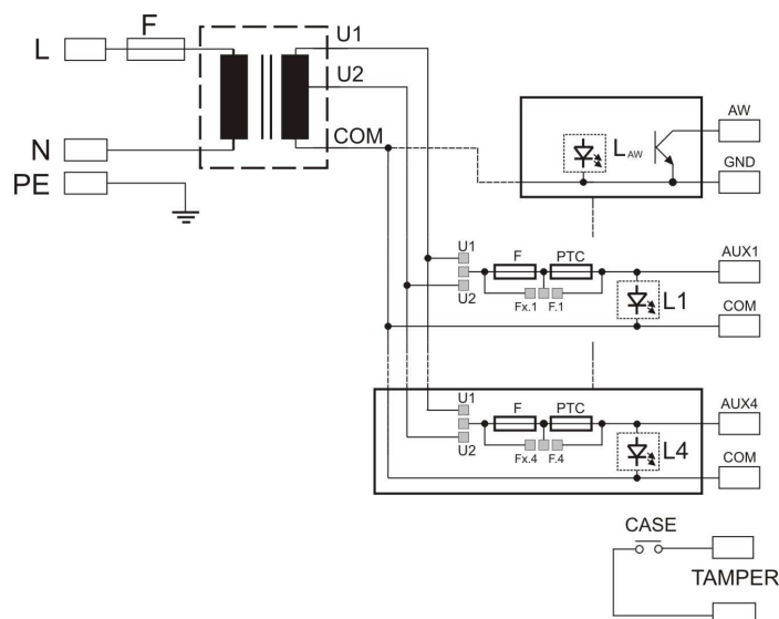
Fig.1. Block diagram of the PSU.
